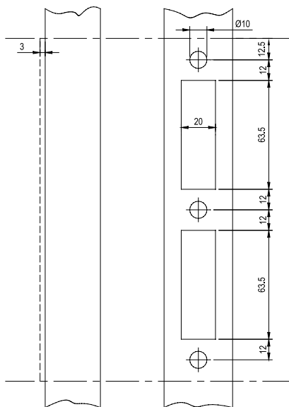
5018/5032 - aluminium frame
