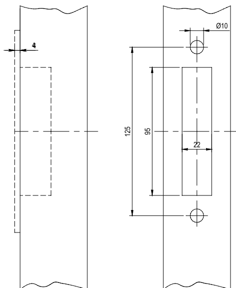
5049 - aluminium frame
